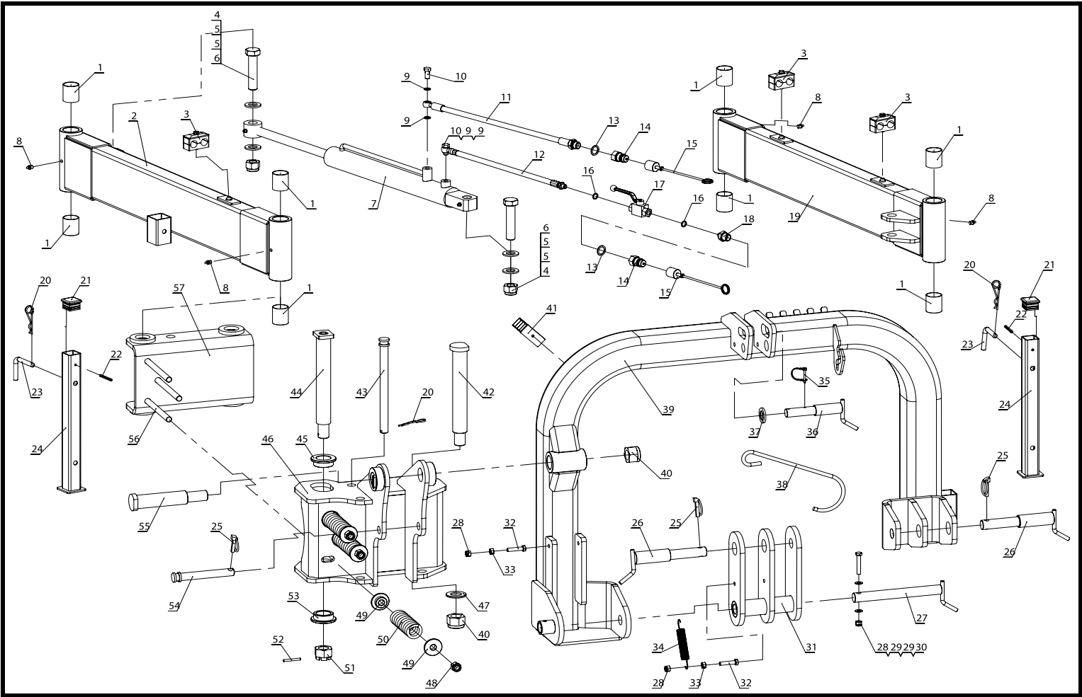
KDL PROFI three-point linkage
