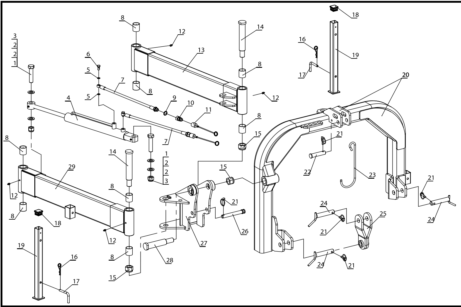
KDL three-point linkage
