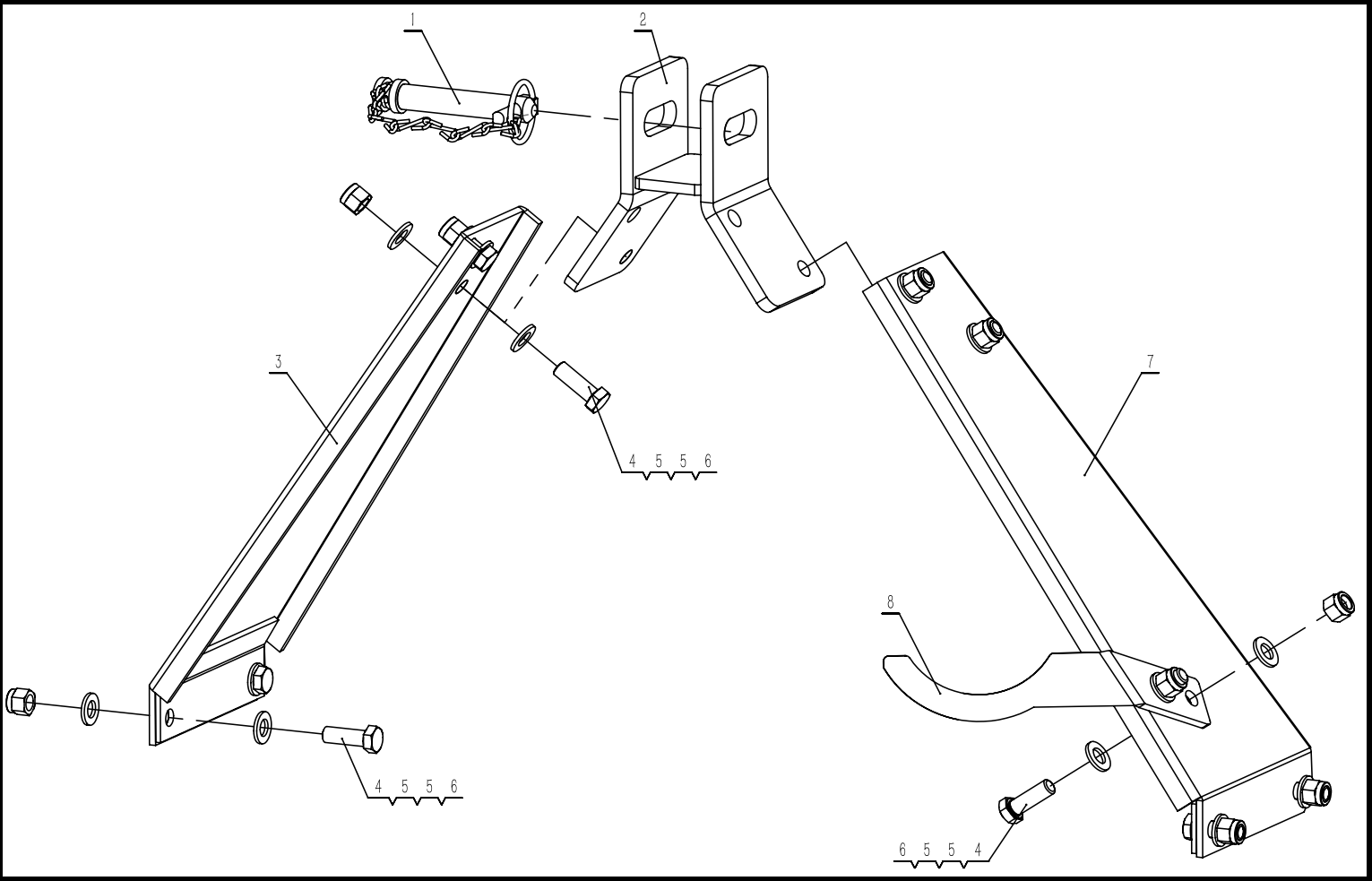
KS three-point linkage
