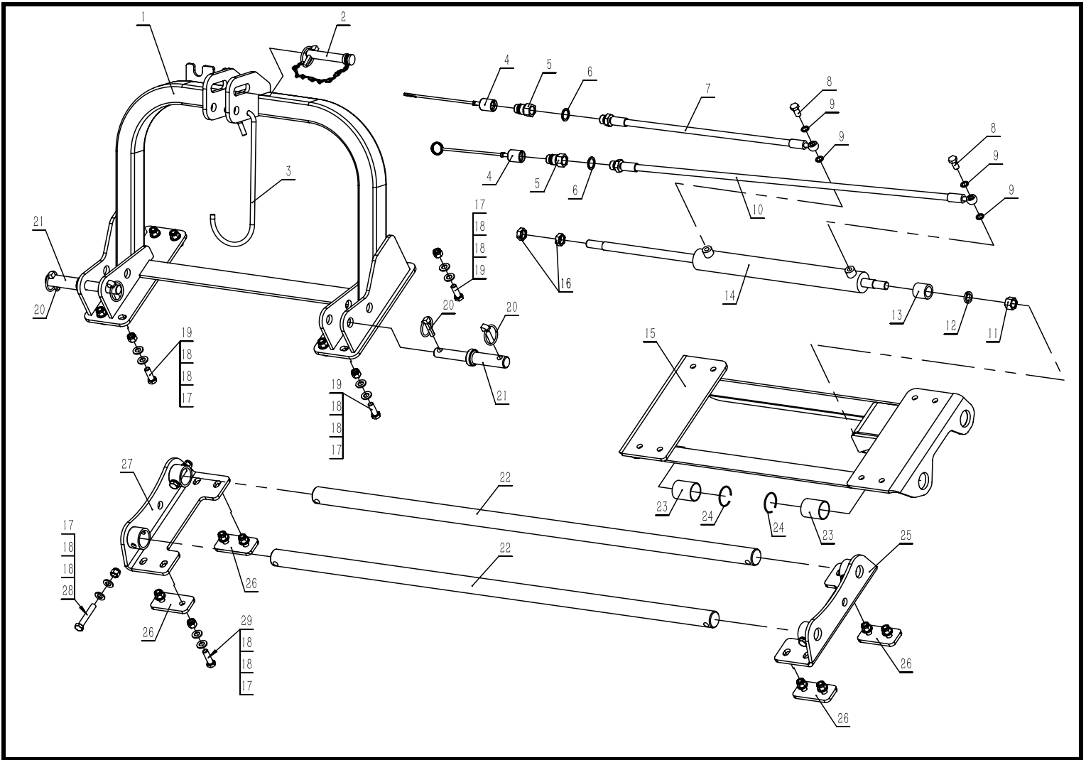
KMH three-point linkage
